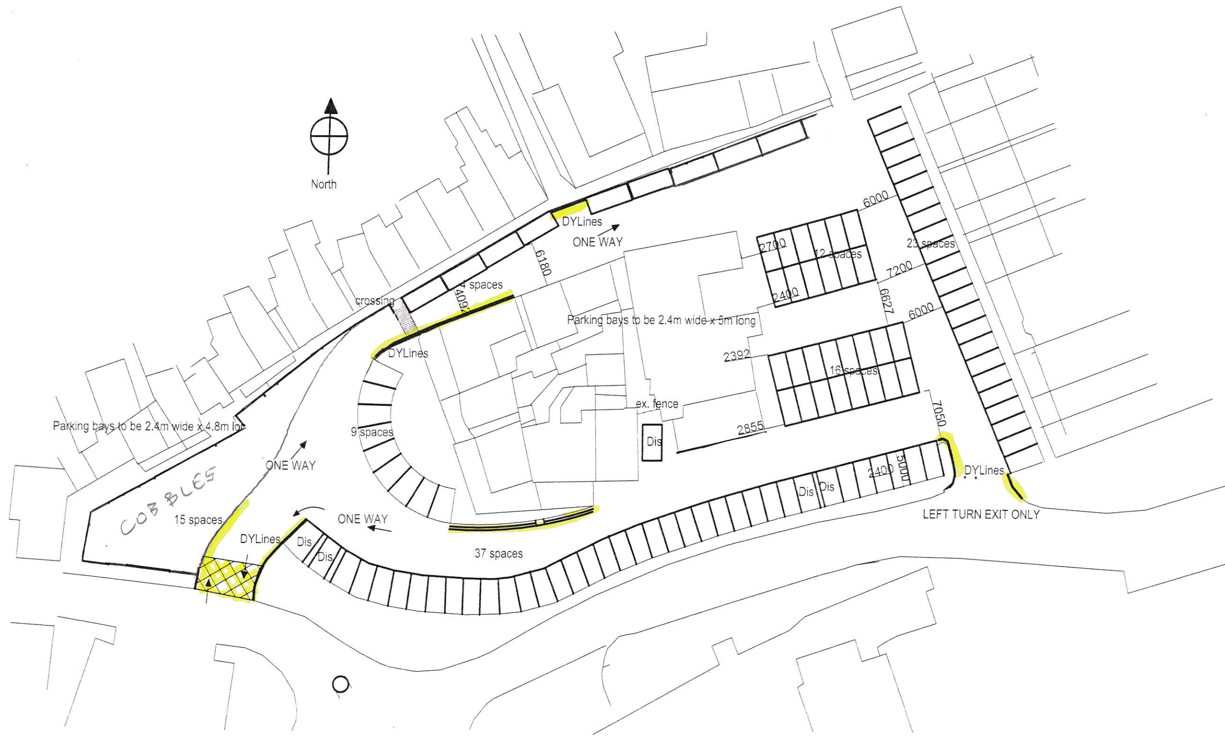
PROPOSED REVISED LAYOUT
